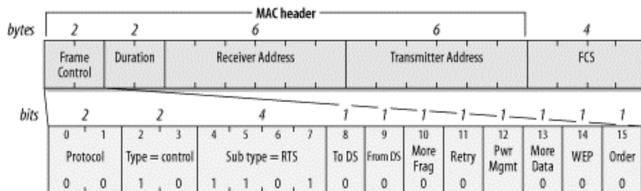
Figure 4-13. RTS frame
