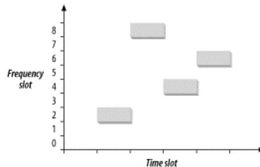
Figure 10-1. Frequency hopping
