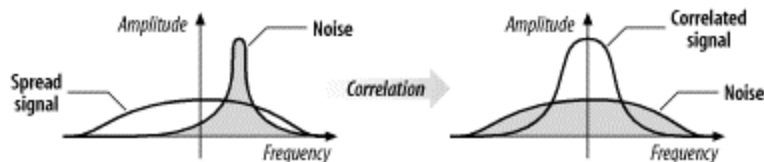
Figure 10-12. Spreading of noise by the correlation process
