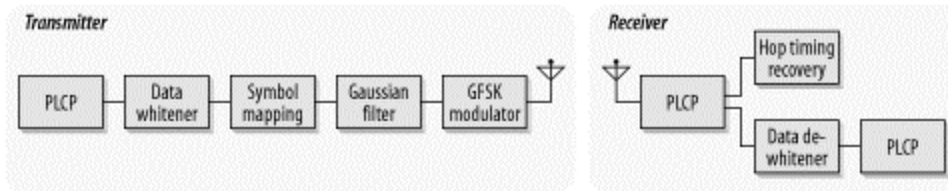
Figure 10-10. Frequency-hopping transceiver
