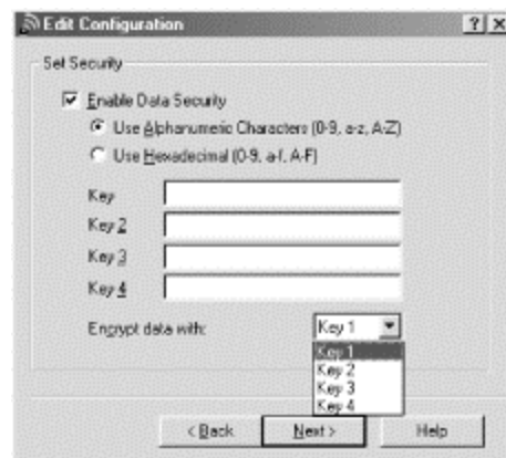
Figure 12-29. WEP configuration
