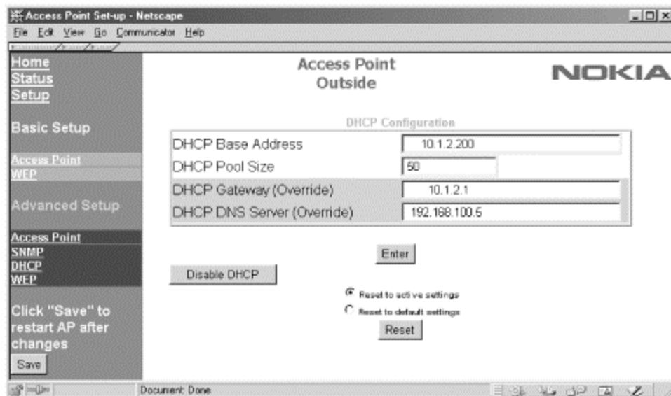
Figure 14-16. DHCP configuration
