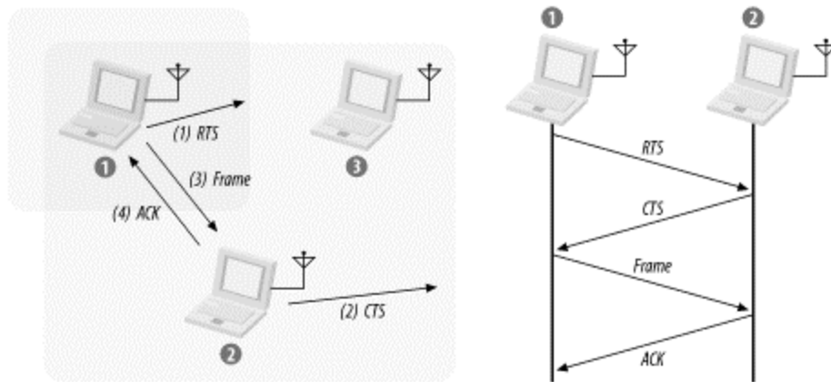
Figure 3-3. RTS/CTS clearing
