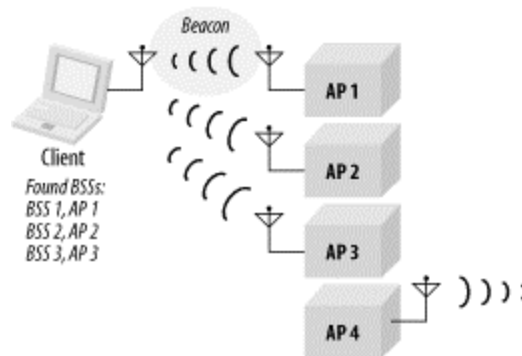
Figure 7-2. Passive scanning
