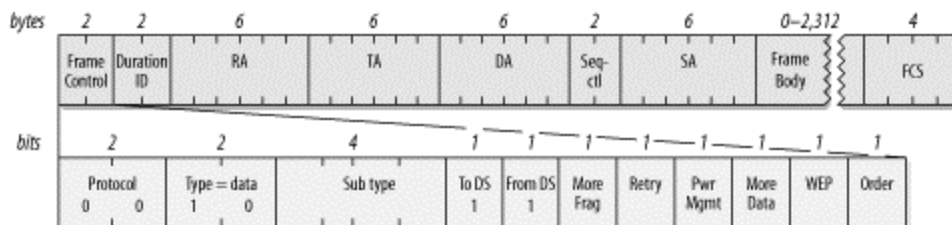
Figure 4-11. WDS frames
