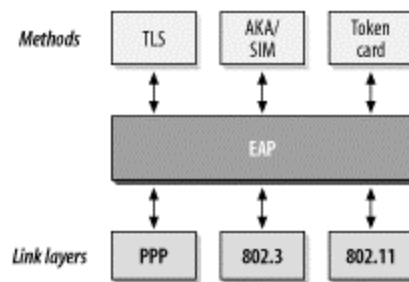
Figure 6-1. EAP architecture
