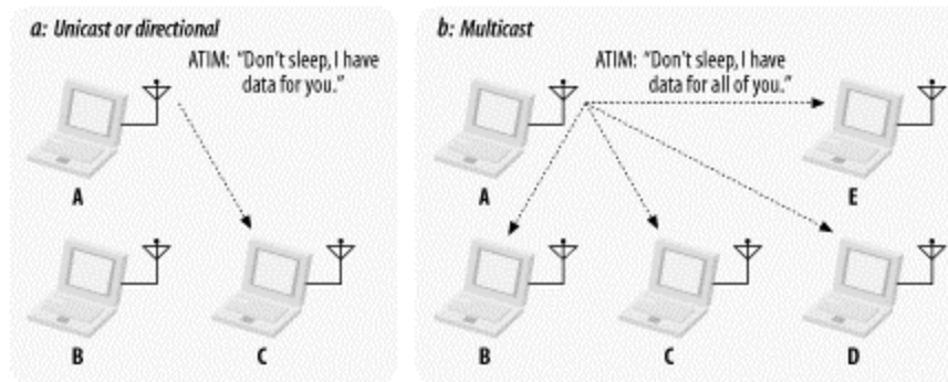
Figure 7-13. ATIM usage
