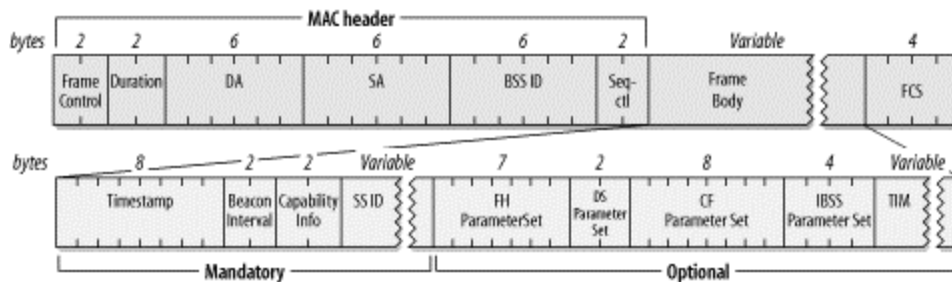
Figure 4-39. Beacon frame
