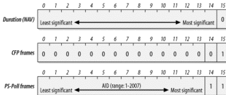
Figure 3-11. Duration/ID field
