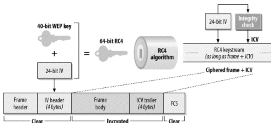
Figure 5-3. WEP operations
